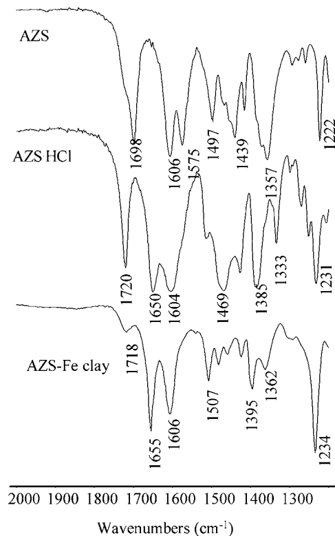
Figure 6. FT-IR spectra of azimsulfuron, azimsulfuron hydrochloride, and azimsulfuron-iron montmorillonite complex.
